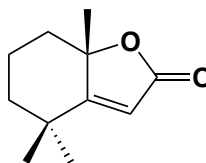
(S)-(+)-Dihydroactinidiolide (2)
