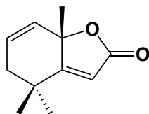
(S)-(+)-Actinidiolide (1)
