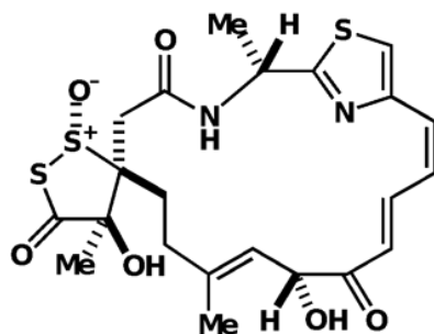
Leinamycin
