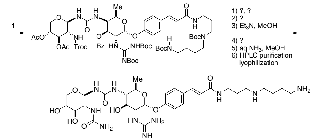
(+)-Glycocinnasperimicin D
